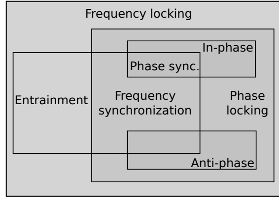
Figure 1.7: Relationship between locking definitions. Adapted from Ref. [17].
