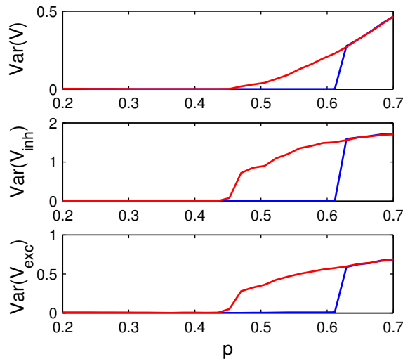
Figure 4.2: Synchronization diagrams for the network of N = 5000 synaptically coupled FHN neurons (4.5). Blue (dark) and red (light) curves show the forward and backward continuations, respectively. The continuation step is \delta p = 0.0075 , the values of other parameters are presented in the text. Equations (4.5) were integrated by Euler-Maruyama method with time step h = 0.05 .
